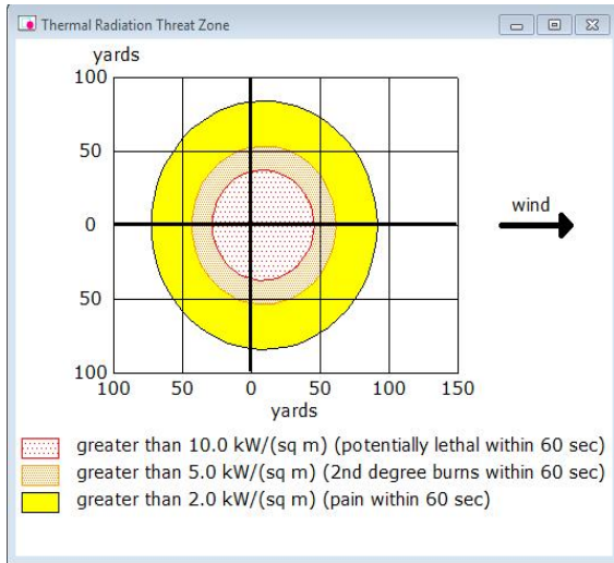
Fig. 8 Thermal effects
