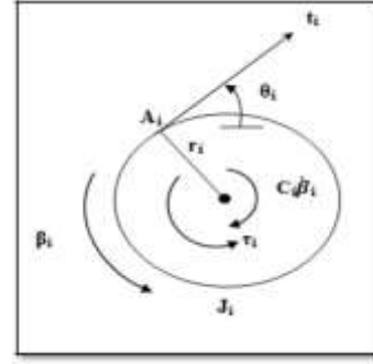
Fig. 3: The structure diagram of the pulley /shaft
