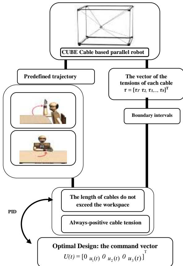
Fig. 4: Optimal design approach for cube- cable based parallel robot for prescribed workspace
