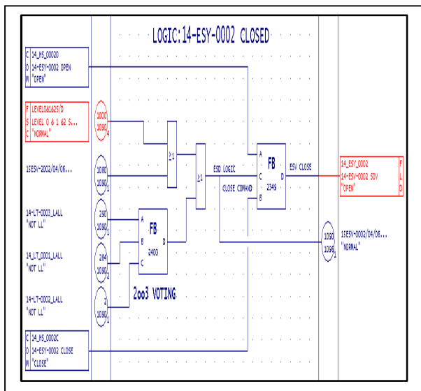
Fig. 7. An overview of the voting 2oo3 implementation on safety manager SIS controller.
