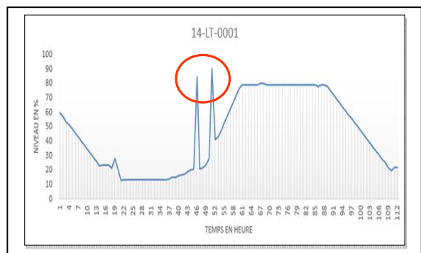
Fig.2. False alarm very high level of 14-LT-0001.
