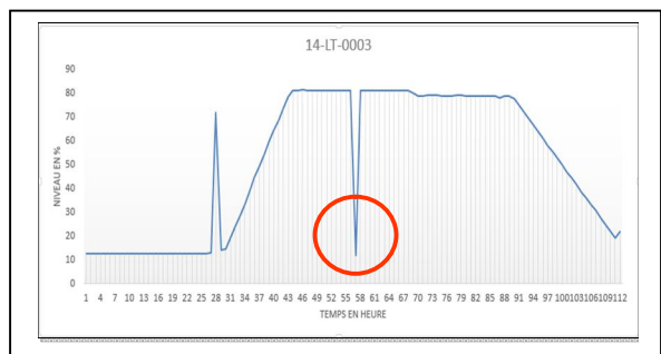
Fig.3. False alarm very low level of 14-LT-0003.
