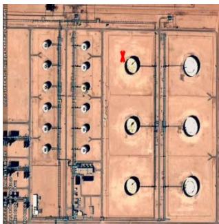
Figure 2: Condensate tank situation
