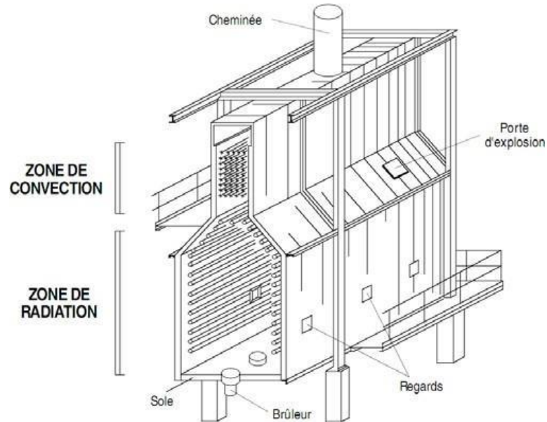
Figure II. 7: Four Classique [23]
