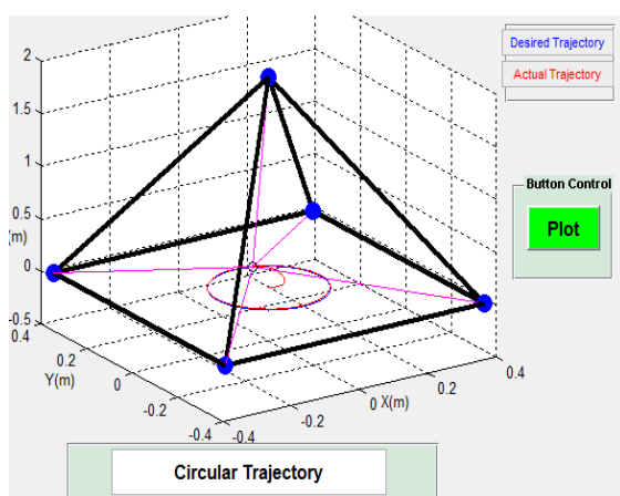
Fig. 10 Plot the desired path and actual path for a circular trajectory.
