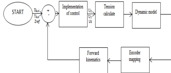
Fig. 3 Control Architecture.
