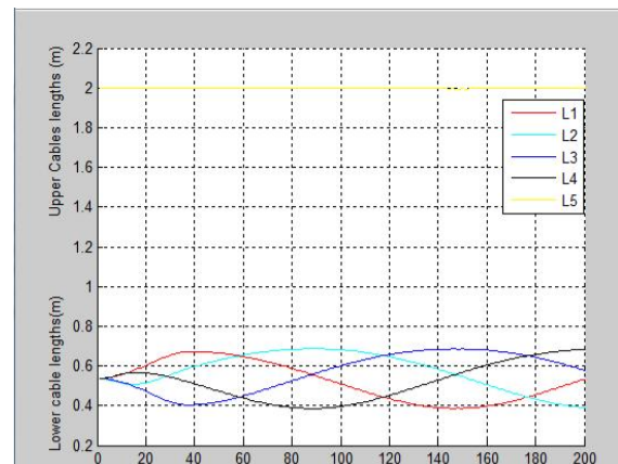
Fig. 11 the cables lengths to draw a circular trajectory in the 2D plane.
