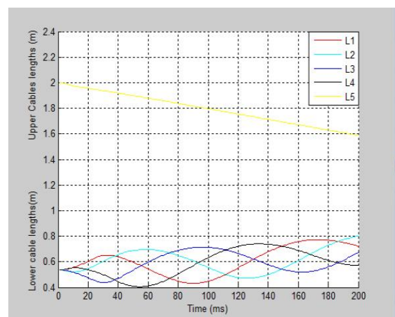
Fig. 13 the cables lengths to draw a spiral trajectory in the 3D plane.
