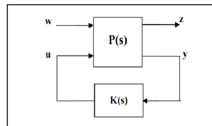
Fig.4. Standard problem (LFT representation)
