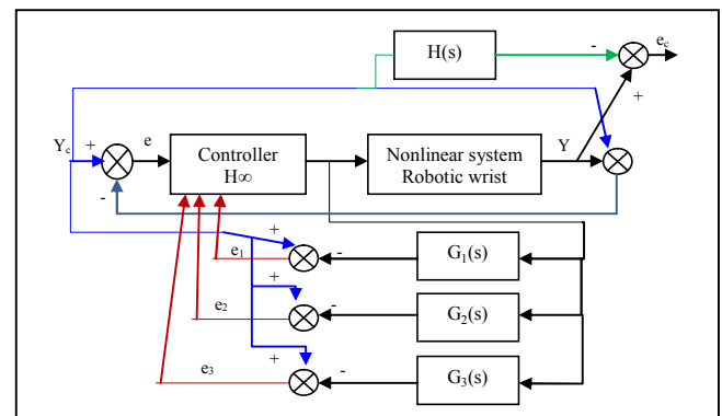
Fig.1. Structure of multi-model approach of control.
