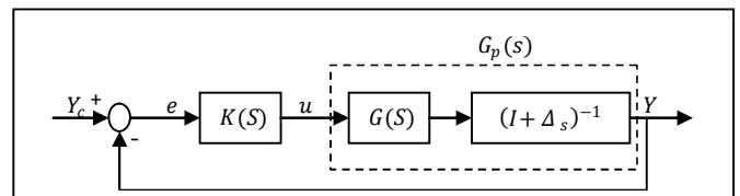
Fig.7. Feedback configuration with inverse output multiplicative uncertainties
