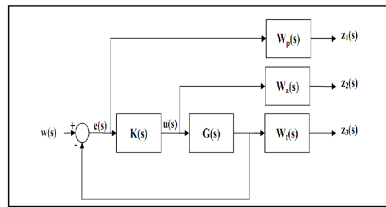
Fig.3. Problem formulation Standard
