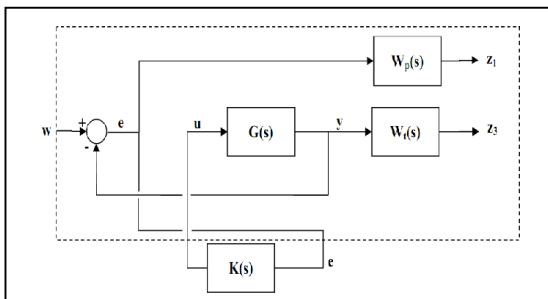
Fig.5. Mixed sensitivity problem in standard form
