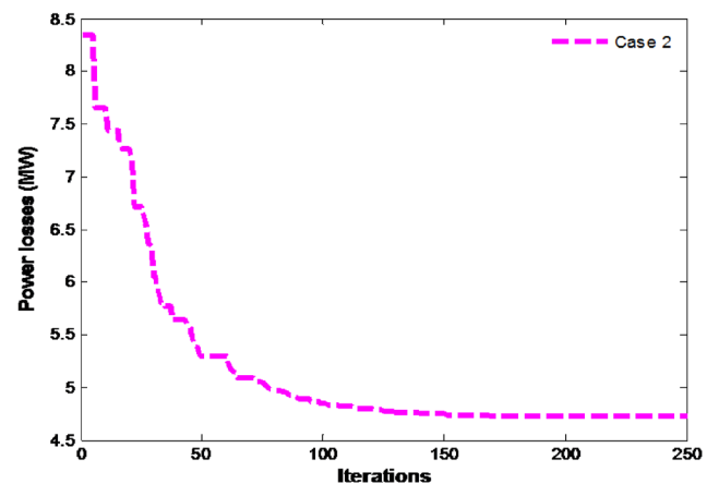
Fig. 3 Convergences of algorithm for case 2
