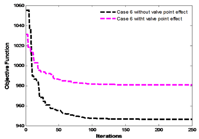
Fig. 7 Convergence of algorithm for case 6
