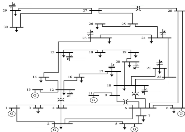
Fig. 1 Single line diagram of IEEE-30 bus system
