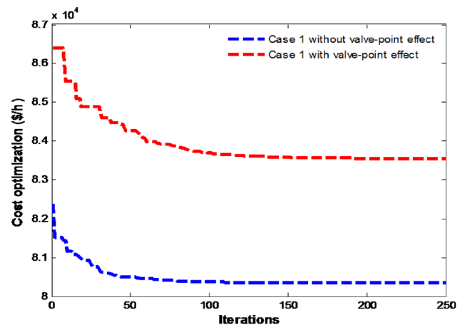
Fig. 2 Convergences of algorithm for case 1
