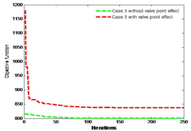
Fig. 6 Convergence of algorithm for case 5
